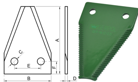
S-SMOOTH, B-BOTTOM SERATED, T-TOP SERRATED
